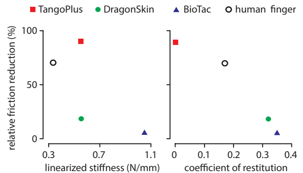
Fig. 9. Friction reduction effectiveness compared to quasi-static stiffness and coefficient of restitution of each finger. Relationship between coefficient of restitution and friction reduction power is monotonic for the sample of fingertips tested.
